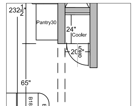
1 Cooler Plan Scale: 1/4" = 1'- 0"
