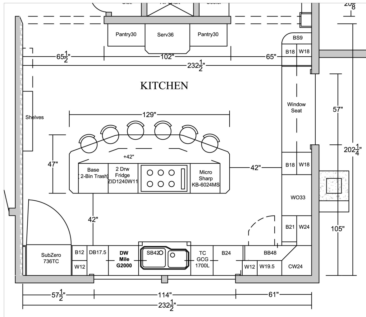
1 Kitchen Plan Scale: 1/4" = 1'-0"
